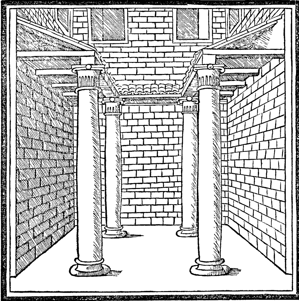
Cauædiū qđ tetraſtylon dicitur
